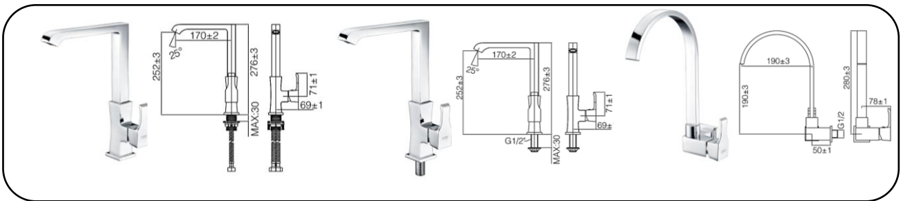
VT5903 Sink Mixer
